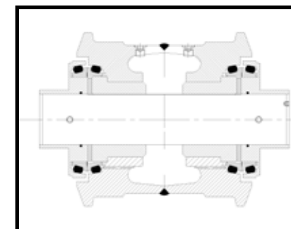
Seal for Tread Roller of Excavator
