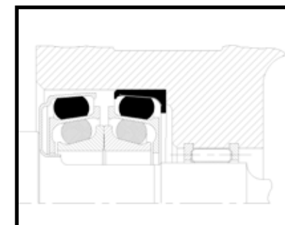
Seal for Steering Drive Axle
