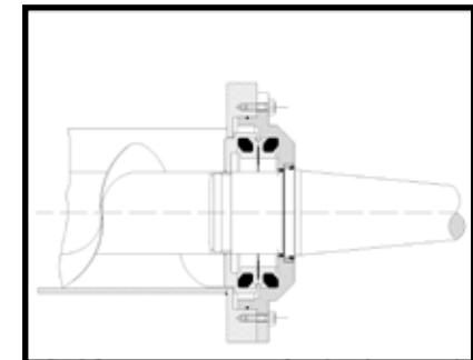
Seal for Screw Conveyor for Abrasive Material
