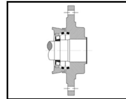
Seal for Rigid Axle of Tractor
