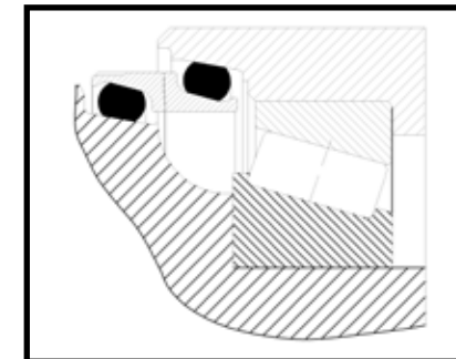
Seal for Wheel Bearing Axle
