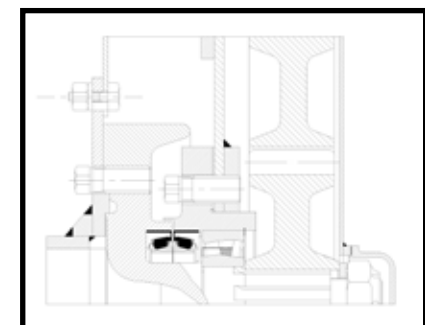
Seal for Transmission Housing
