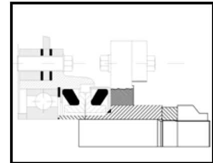
Seal for Cutting Shaft of Crop Harvester
